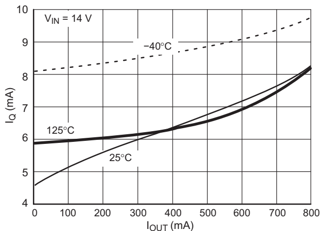
Figure 7. Quiescent Current vs. Output Current Over Temperature
