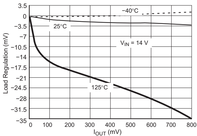
Figure 5. Load Regulation vs. Output Current Over Temperature
