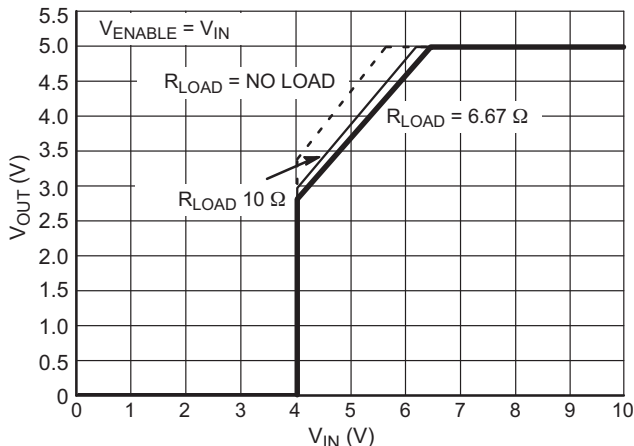
Figure 2. V_{OUT} vs. V_{IN} over R_{LOAD} ; T = 25^{\circ}C
