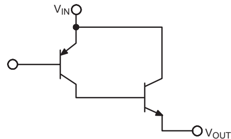
Figure 14. Composite Output Stage of the CS8140/1
