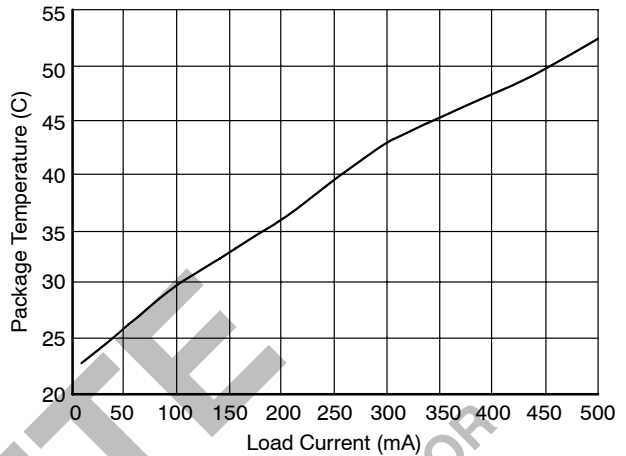
Figure 25. Package Temperature vs. Load Current ( V_{IN} = 5.0 V , T_A = 23^\circ C )
