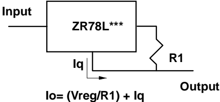
Current Regulator
