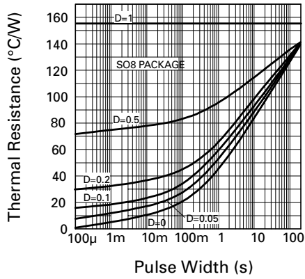
Thermal Resistance v Pulse Width
