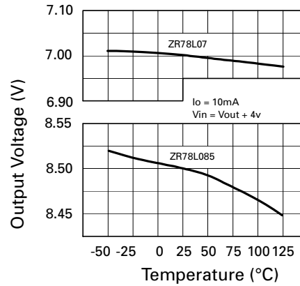
Output Voltage Temperature Coefficient
