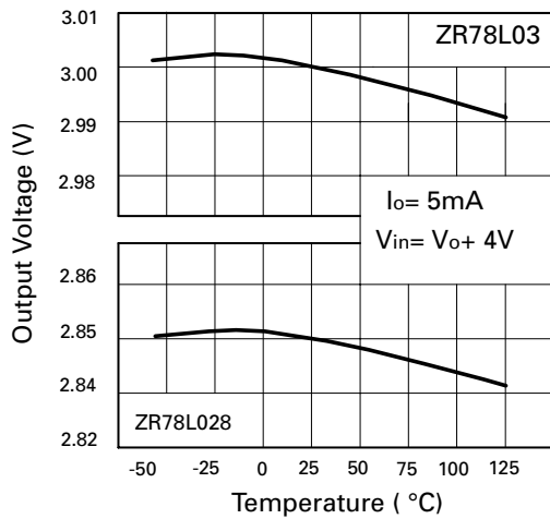
Output Voltage Temperature Coefficient
