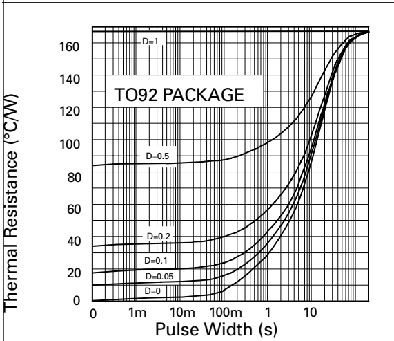
Thermal Resistance v Pulse Width
