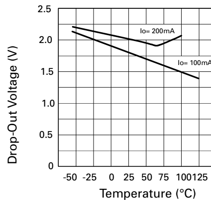
Drop-Out Voltage v Temperature
