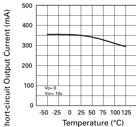
Peak Output Current v Temperature
