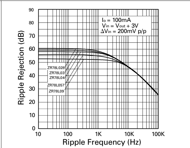
Ripple Rejection vs. Ripple Frequency
