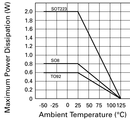
Power dissipation Derating
