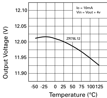
Output Voltage Temperature Coefficient
