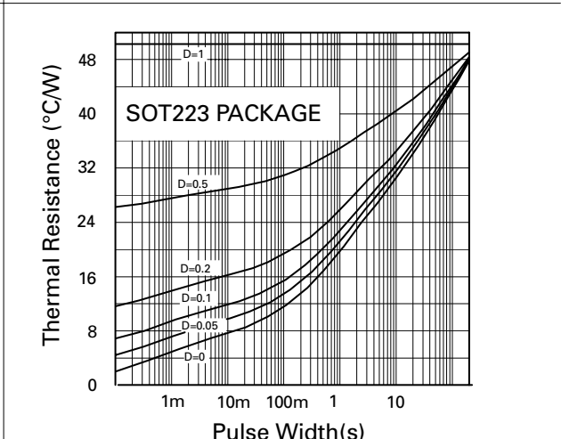
Thermal Resistance v Pulse Width
