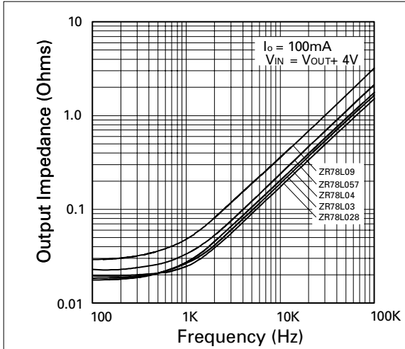
Output Impedance vs. Frequency
