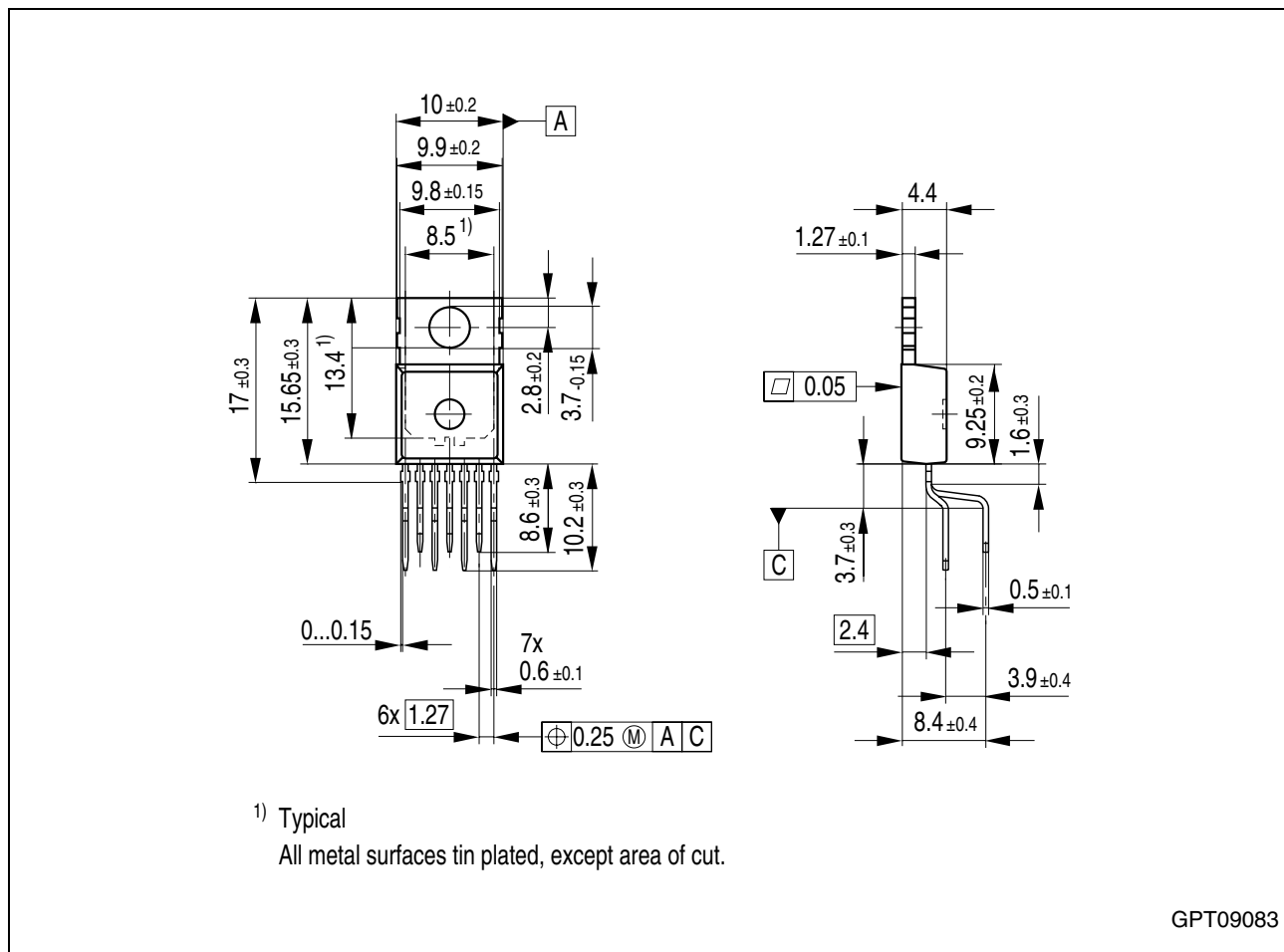
Figure 8 PG-TO220-7-11 (Plastic Transistor Single Outline)
