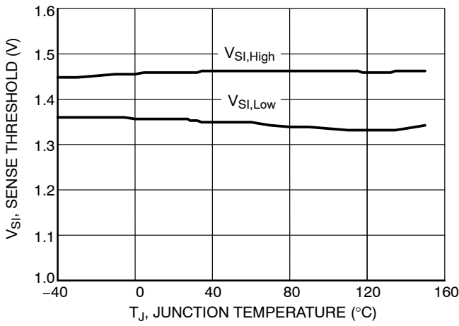
Figure 10. Sense Threshold vs. Junction Temperature
