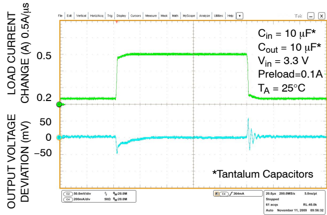
Figure 31. Load Transient Response – V_{out} = 5.0V
