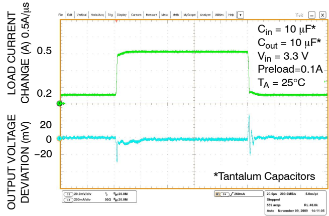
Figure 29. Load Transient Response – V_{out} = 2.5V
