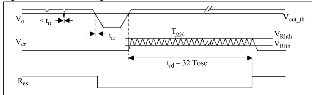
Figure 27. Reset time diagram
