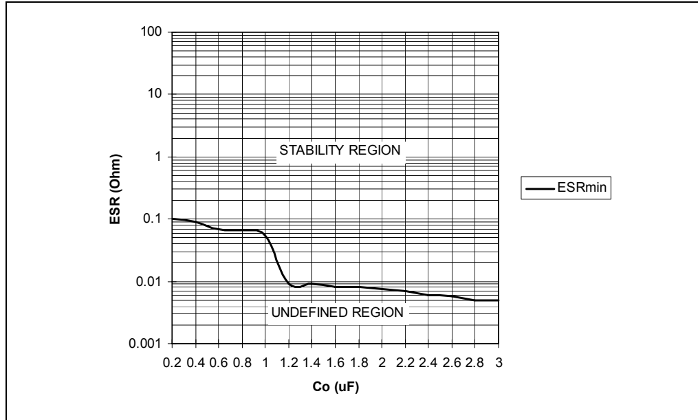
Figure 25. Stability region (1)
