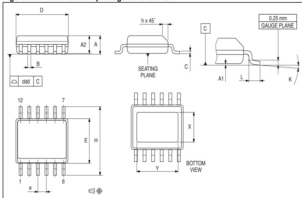
Figure 33. PowerSSO-12 package dimensions
