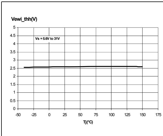
Figure 19. V_{EWi\_thh} vs. T_j
