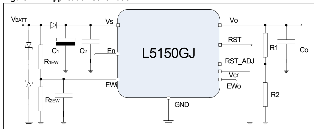
Figure 24. Application schematic
