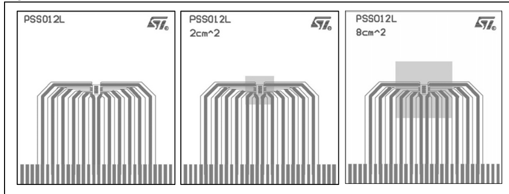
Figure 29. PowerSSO-12 PC board (1)
