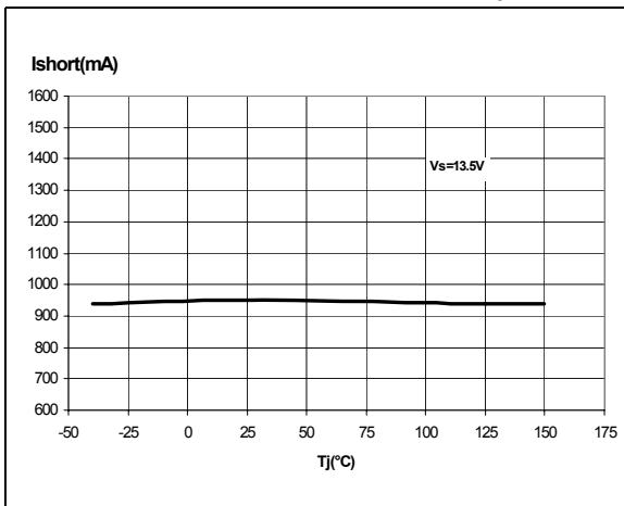
Figure 13. Short-circuit current vs. T_j
