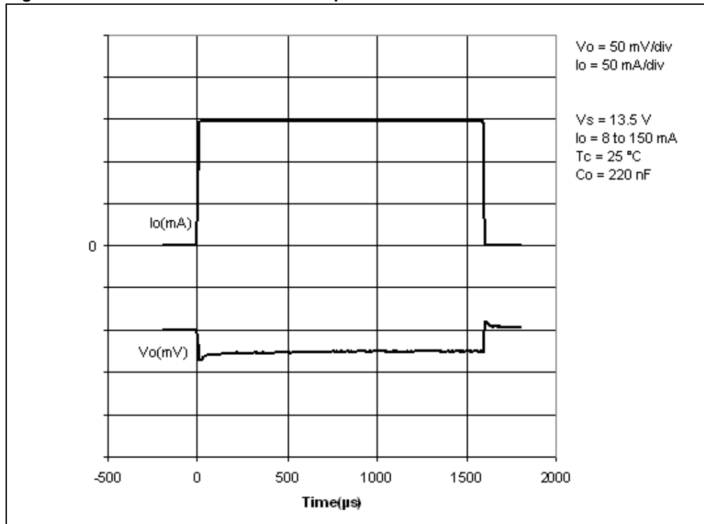
Figure 26. Maximum load variation response
