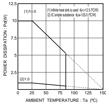
Fig.8 Thermal derating curves (TO252-5)
