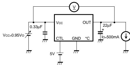
Fig.3 Measurement circuit for minimum I/O voltage differential
