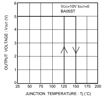
Fig.9 Thermal cutoff circuit characteristics
