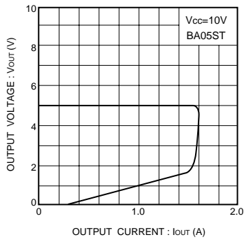
Fig.10 Current limit characteristics
