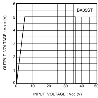
Fig.11 Over voltage protection characteristics
