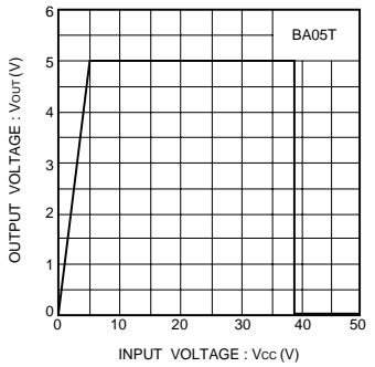
Fig. 10 Over voltage protection characteristics
