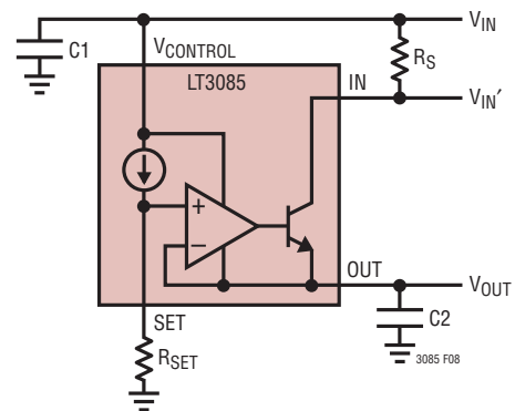
Figure 8. Reducing Power Dissipation Using a Series Resistor
