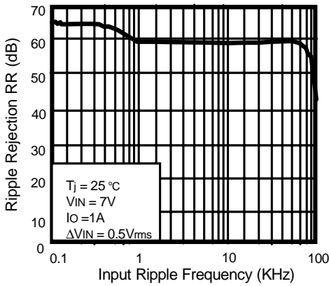
Figure 9. Ripple Rejection vs. Input Ripple Frequency
