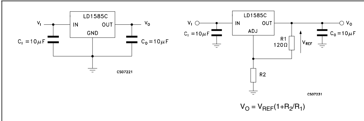
Figure 3. Application circuits
