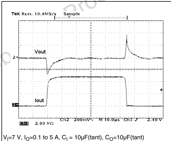
Figure 26. Load transient
