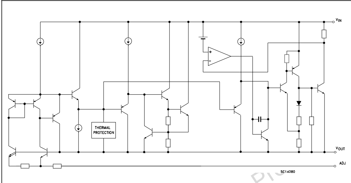
Figure 1. Schematic diagram
