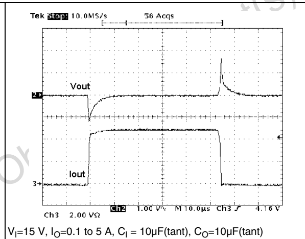
Figure 25. Load transient
