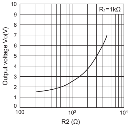
Fig.14 Output Voltage Adjustment Characteristics (Typical value)
