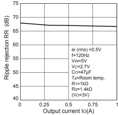
Fig.12 Ripple Rejection vs. Output Current
