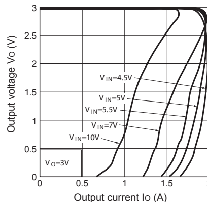
Fig.4 Overcurrent Protection Characteristics
