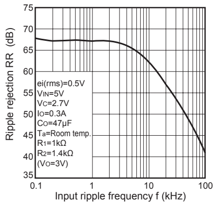
Fig.11 Ripple Rejection vs. Input Ripple Frequency
