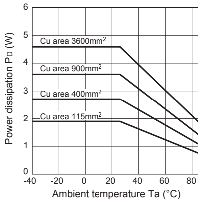
Fig.13 Power Dissipation vs. Ambient Temperature
