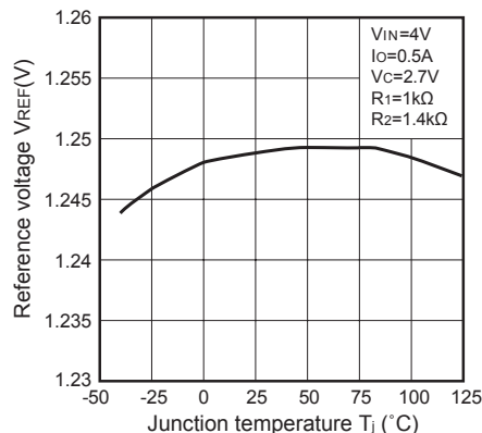
Fig.5 Reference Voltage vs. Junction Temperature
