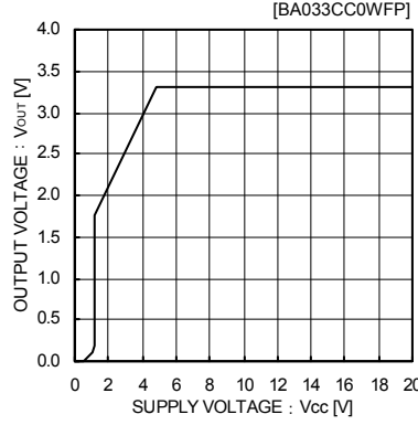
Fig.2 Input Stability
