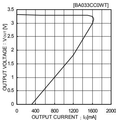
Fig.4 Load Stability
