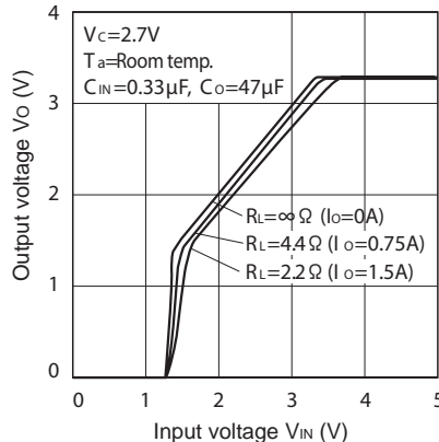
Fig.18 Output Voltage vs. Input Voltage (PQ033EZ1HZxH)
