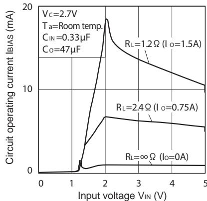
Fig.20 Circuit Operating Current vs. Input Voltage (PQ018EZ1HZxH)
