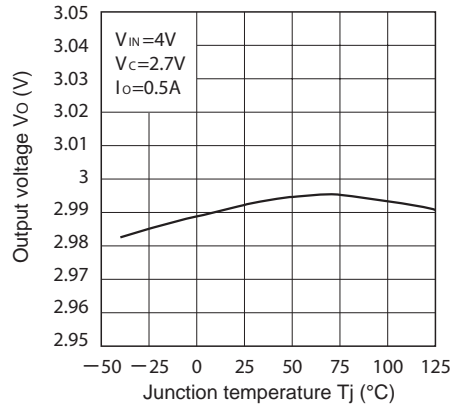
Fig.12 Output Voltage vs. Junction Temperature (PQ030EZ1HZxH)
