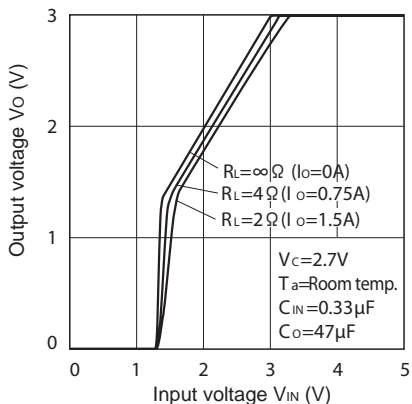
Fig.17 Output Voltage vs. Input Voltage (PQ030EZ1HZxH)
