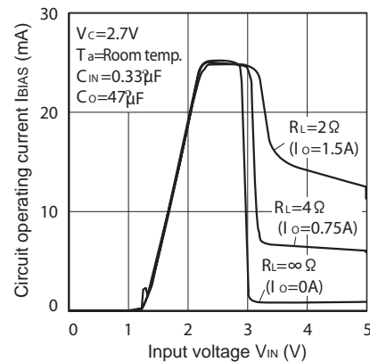
Fig.22 Circuit Operating Current vs. Input Voltage (PQ030EZ1HZxH)
