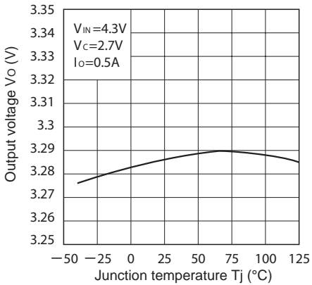
Fig.13 Output Voltage vs. Junction Temperature (PQ033EZ1HZxH)
