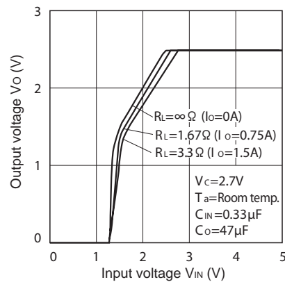
Fig.16 Output Voltage vs. Input Voltage (PQ025EZ1HZxH)
