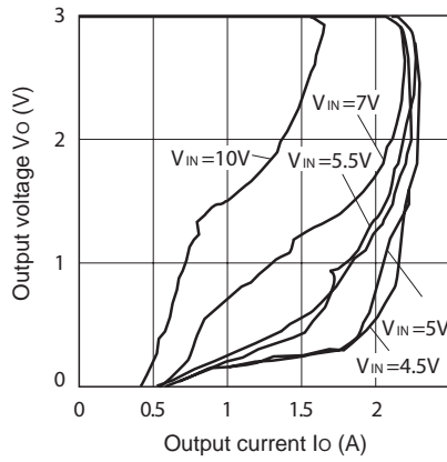
Fig.7 Overcurrent Protection Characteristics (PQ030EZ1HZxH)
