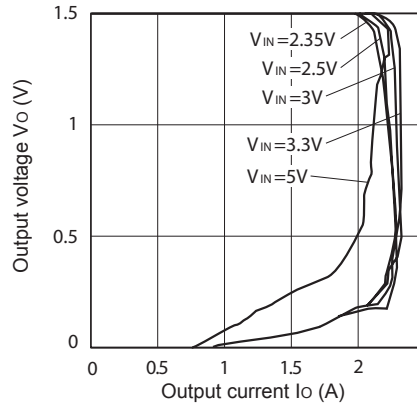
Fig.4 Overcurrent Protection Characteristics (PQ015EZ1HZxH)
