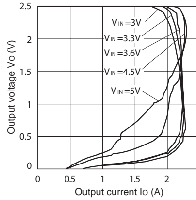
Fig.6 Overcurrent Protection Characteristics (PQ025EZ1HZxH)
