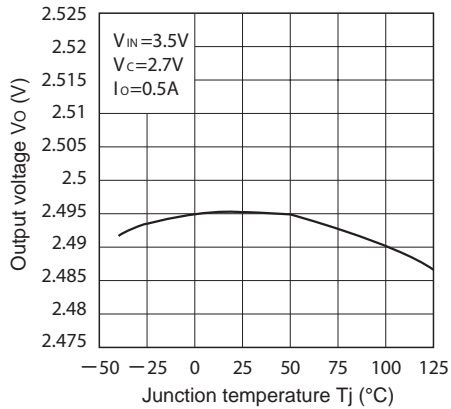
Fig.11 Output Voltage vs. Junction Temperature (PQ025EZ1HZxH)
