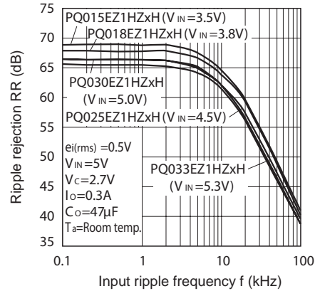
Fig.26 Ripple Rejection vs. Input Ripple Frequency
