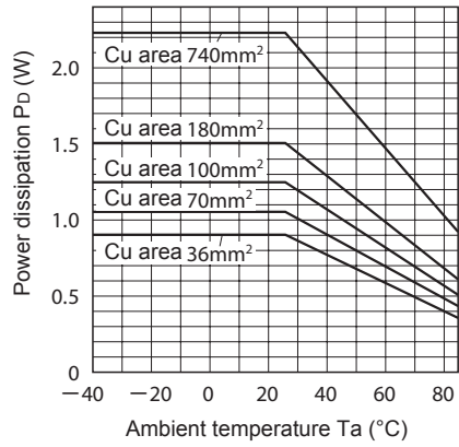
Fig.28 Power Dissipation vs. Ambient Temperature (Typical Value)
