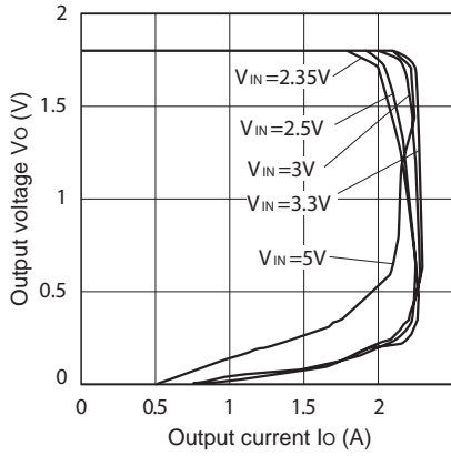
Fig.5 Overcurrent Protection Characteristics (Typical Value)(PQ018EZ1HZxH)
