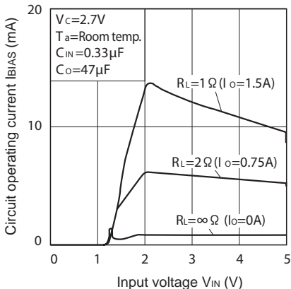
Fig.19 Circuit Operating Current vs. Input Voltage (PQ015EZ1HZxH)
