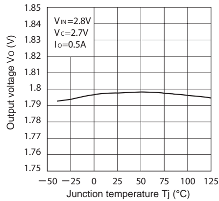
Fig.10 Output Voltage vs. Junction Temperature (PQ018EZ1HZxH)
