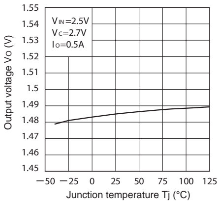
Fig.9 Output Voltage vs. Junction Temperature (PQ015EZ1HZxH)
