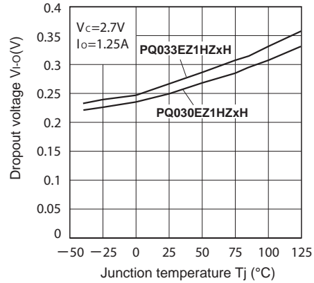
Fig.24 Dropout Voltage vs. Junction Temperature
