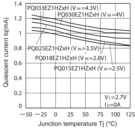
Fig.25 Quiescent Current vs. Junction Temperature
