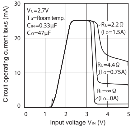
Fig.23 Circuit Operating Current vs. Input Voltage (PQ033EZ1HZxH)
