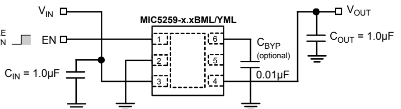
Ultra-Low Noise Regulator Application
