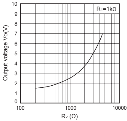
Fig.14 Output Voltage Adjustment Characteristics
