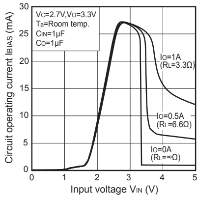
Fig.9 Circuit Operating Current vs. Input Voltage
