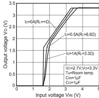
Fig.8 Output Voltage vs. Input Voltage
