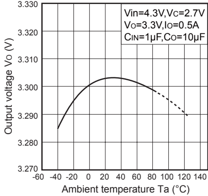
Fig.5 Output Voltage vs. Ambient Temperature
