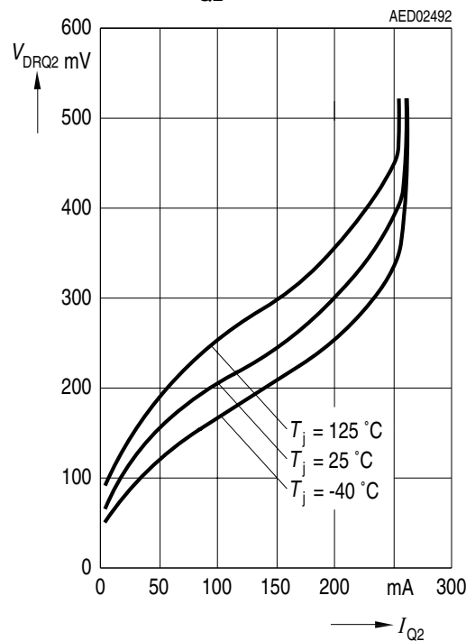
Drop Voltage V_{DRQ2} versus Output Current I_{Q2}
