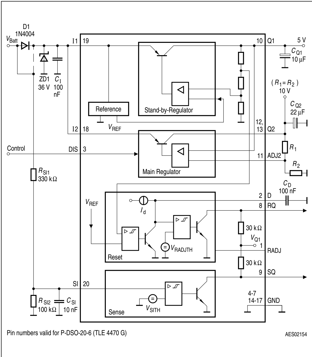
Figure 3 Application Circuit
