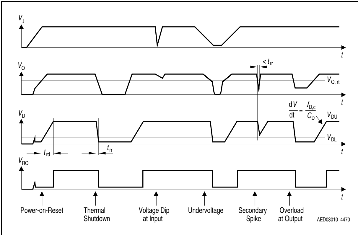
Figure 4 Reset Timing
