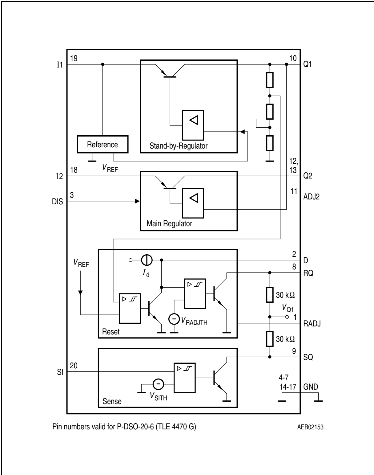
Figure 2 Block Diagram
