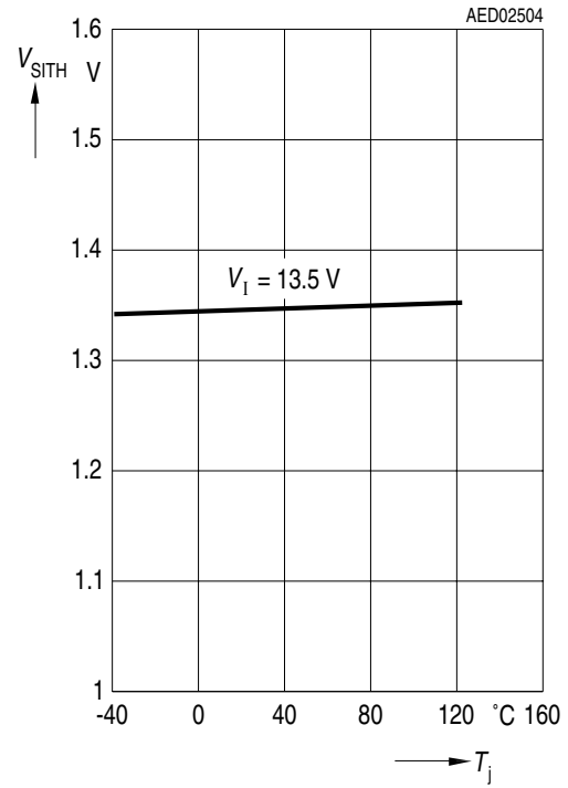
Sense Threshold V_{SITH} versus Temperature T_j
