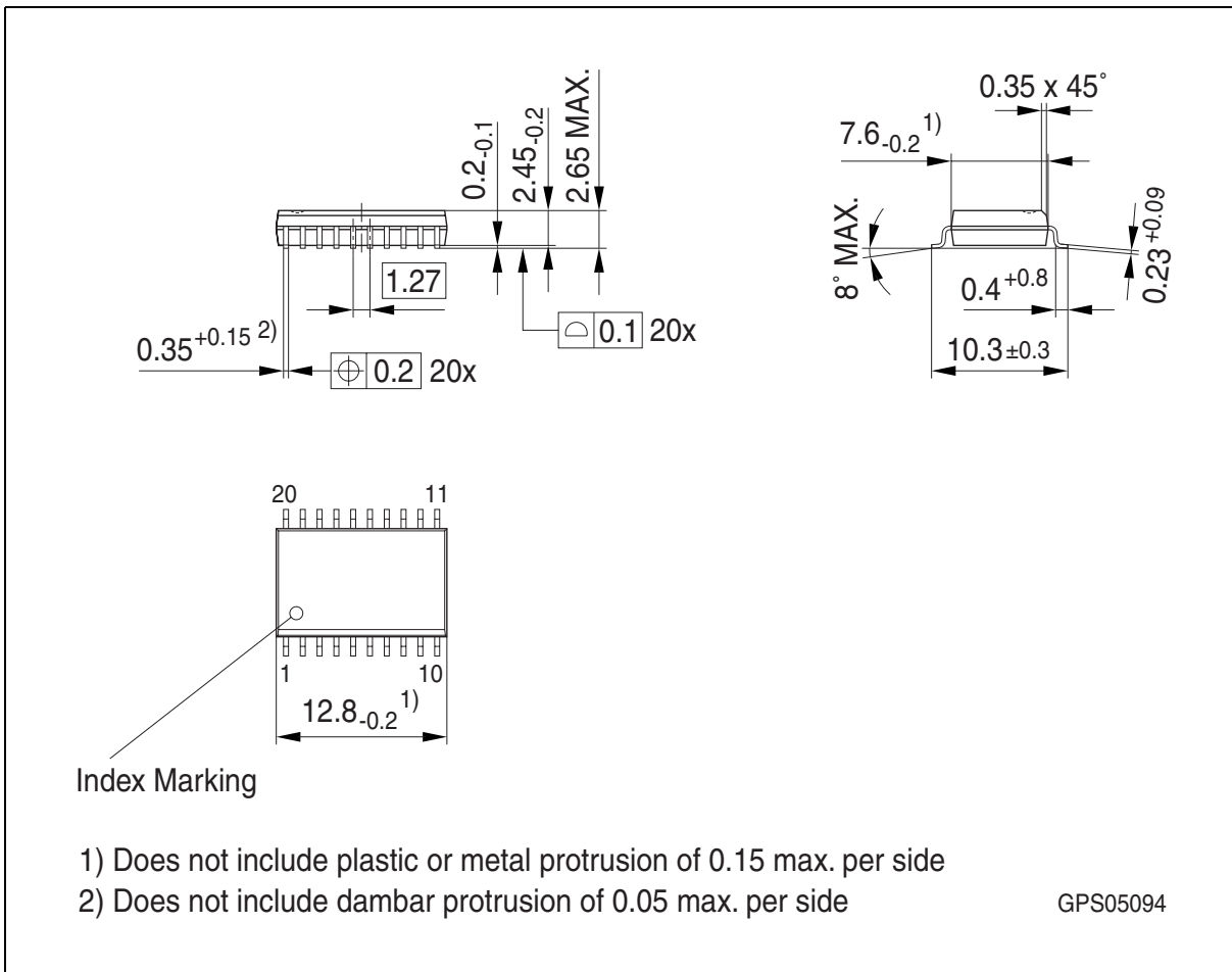
Figure 7 PG-DSO-20 (Plastic Green Dual Small Outline)
