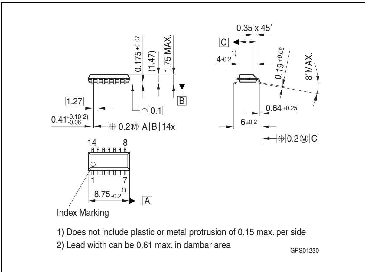
Figure 6 PG-DSO-14 (Plastic Green Dual Small Outline)
