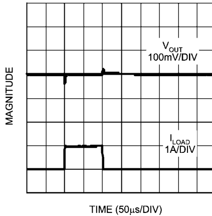
Load Transient Response C_{IN} = C_{OUT} = 100\mu F , POSCAP
