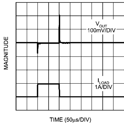
Load Transient Response C_{IN} = C_{OUT} = 10\mu F , TANTALUM
