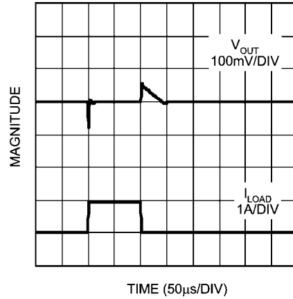
Load Transient Response C_{IN} = C_{OUT} = 10\mu F , OSCON
