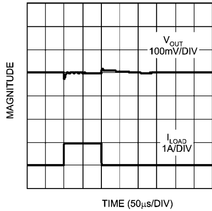
Load Transient Response C_{IN} = C_{OUT} = 100\mu F , OSCON
