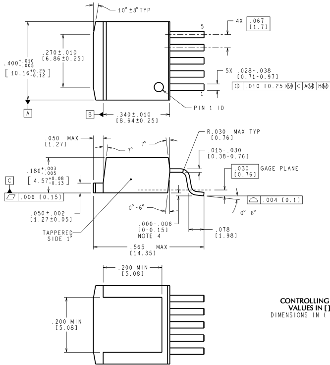
TO263 5-Lead, Molded, Surface Mount Package (TO263-5) NS Package Number TS5B
