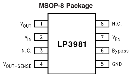
Top View See NS Package Number MUA008AE
