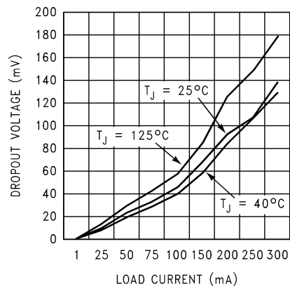
Dropout Voltage vs. Temperature ( V_{OUT} = 2.85V )
