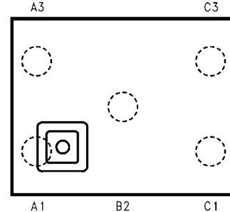
micro SMD, 5 Bump Package
