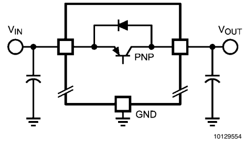
FIGURE 3. Reverse Current Parth
