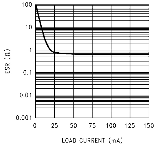
FIGURE 2. LP2985LV 4.7 \mu\text{F} Stable ESR Range
