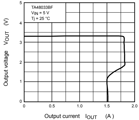
V OUT - I OUT
