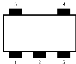
SOT-23, 5-Lead Small Outline Package (M5)
