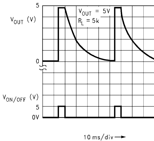
Turn-Off Waveform
