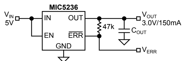
Regulator with Error Output
