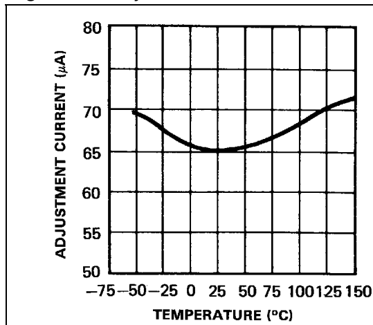
Figure 7. Temperature stability
