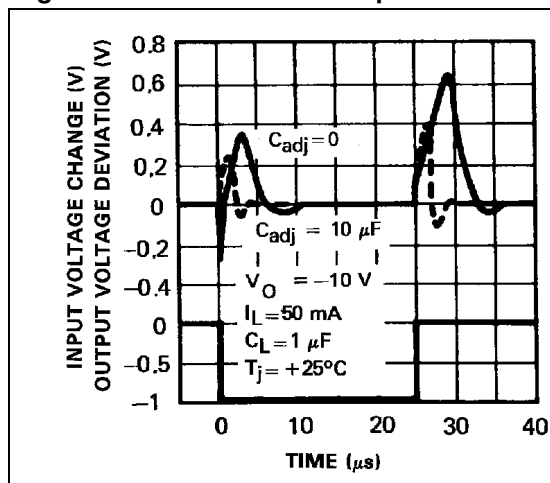
Figure 13. Line transient response
