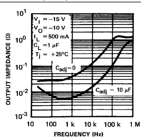
Figure 12. Output impedance
