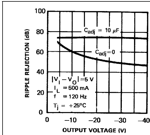
Figure 9. Ripple rejection vs output voltage
