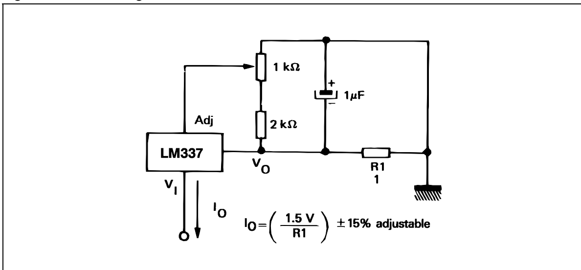
Figure 20. Current regulator
