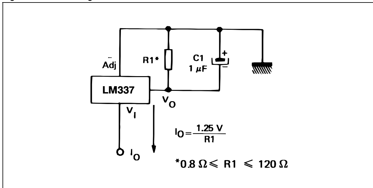
Figure 17. Current regulator
