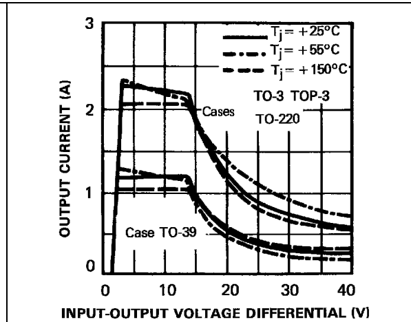
Figure 4. Current limit
