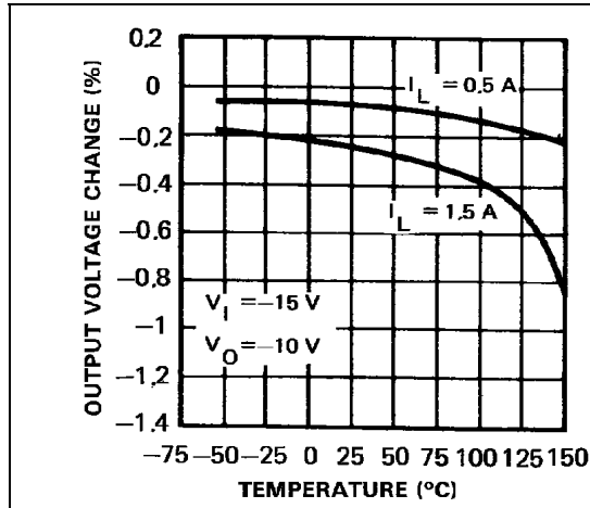
Figure 3. Load regulation
