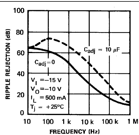
Figure 10. Ripple rejection vs frequency
