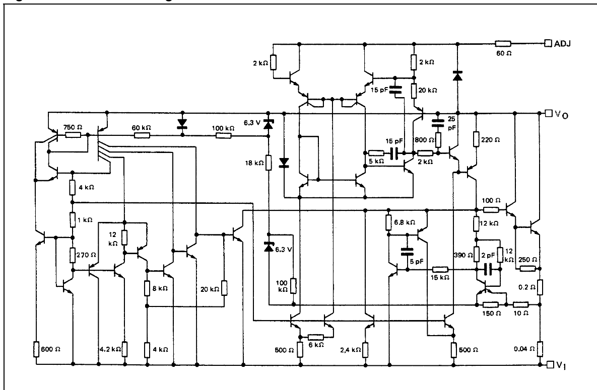
Figure 1. Schematic diagram
