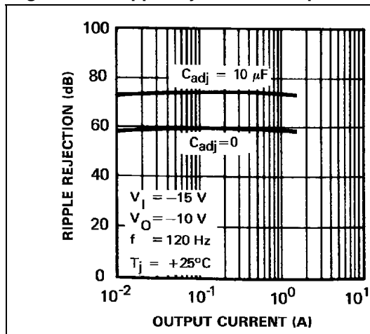
Figure 11. Ripple rejection vs output current
