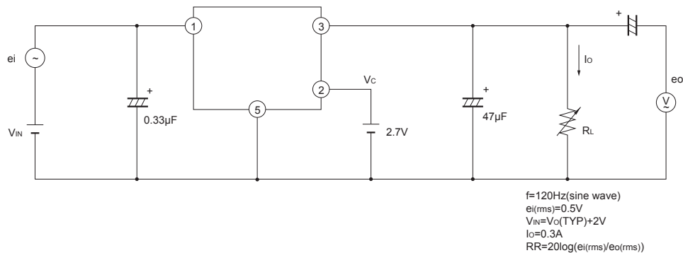
Fig.2 Test circuit of Ripple Rejection
