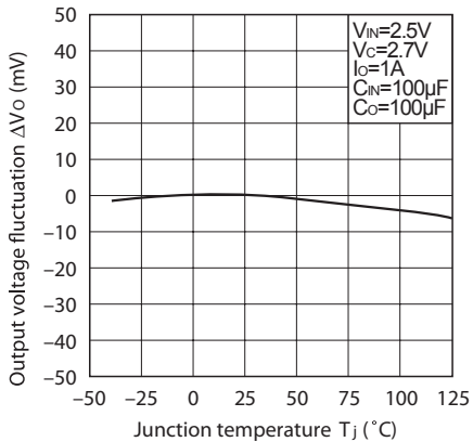
Fig.7 Output Voltage Fluctuation vs. Junction Temperature (PQ015EH02ZxH)
