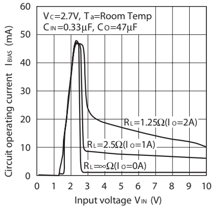
Fig.15 Circuit Operating Current vs. Input Voltage (PQ025EH02ZxH)
