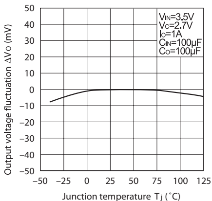
Fig.9 Output Voltage Fluctuation vs. Junction Temperature (PQ025EH02ZxH)
