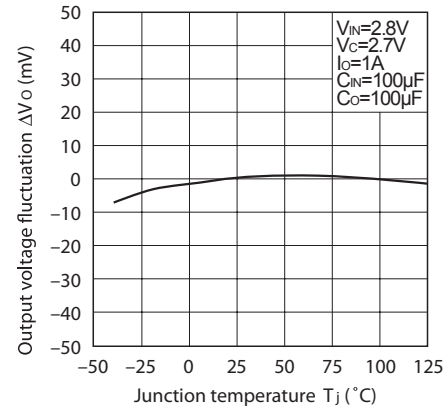
Fig.8 Output Voltage Fluctuation vs. Junction Temperature (PQ018EH02ZxH)
