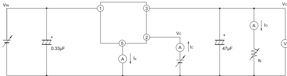
Fig.1 Test Circuit
