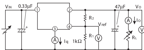
Fig.1 Test Circuit
