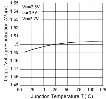
Fig.8 Output Voltage Fluctuation vs. Junction Temperature (PQ015EF01SZH)
