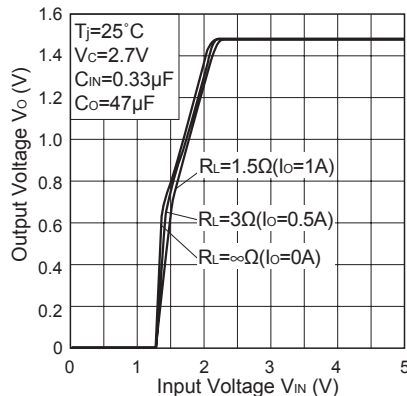
Fig.12 Output Voltage vs. Input Voltage (PQ015EF01SZH)
