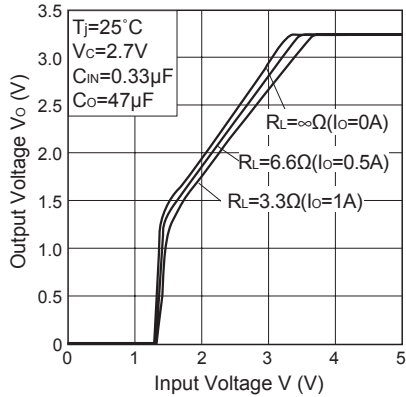
Fig.15 Output Voltage vs. Input Voltage (PQ033EF01SZH)
