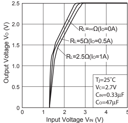
Fig.14 Output Voltage vs. Input Voltage (PQ025EF01SZH)
