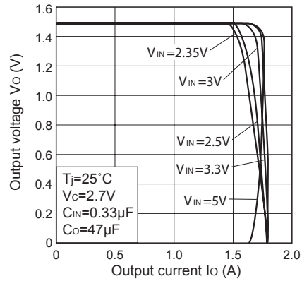
Fig.4 Overcurrent Protection Characteristics (Typical Value, PQ015EF01SZH)
