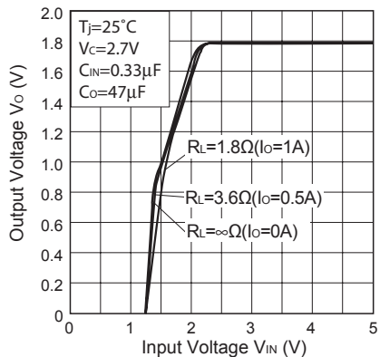
Fig.13 Output Voltage vs. Input Voltage (PQ018EF01SZH)
