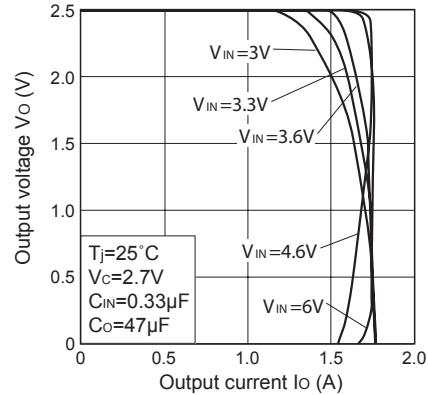
Fig.6 Overcurrent Protection Characteristics (Typical Value, PQ025EF01SZH)
