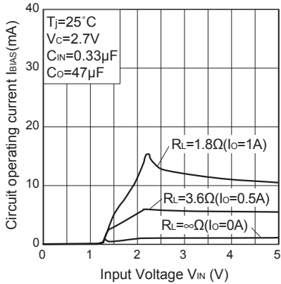
Fig.17 Circuit Operating Current vs. Input Voltage (PQ018EF01SZH)
