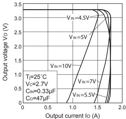
Fig.7 Overcurrent Protection Characteristics (Typical Value, PQ033EF01SZH)
