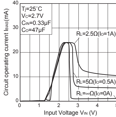
Fig.18 Circuit Operating Current vs. Input Voltage (PQ025EF01SZH)
