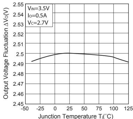
Fig.10 Output Voltage Fluctuation vs. Junction Temperature (PQ025EF01SZH)
