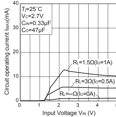
Fig.16 Circuit Operating Current vs. Input Voltage (PQ015EF01SZH)
