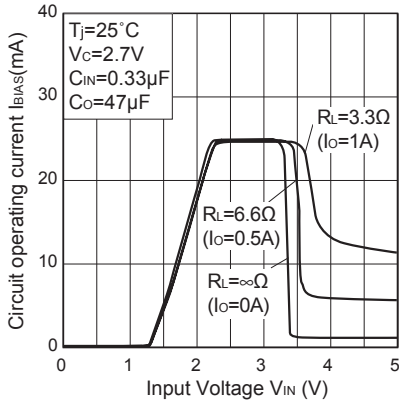
Fig.19 Circuit Operating Current vs. Input Voltage (PQ033EF01SZH)
