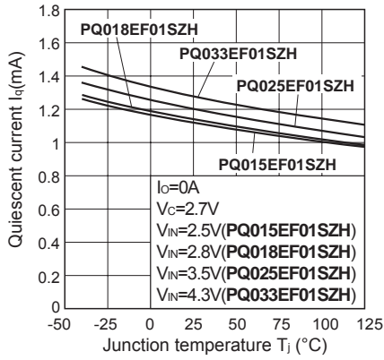
Fig.21 Quiescent Current vs. Junction Temperature
