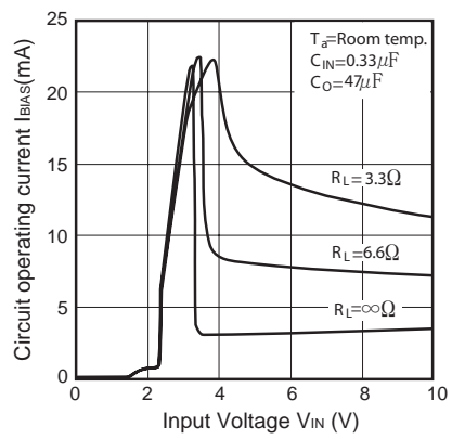
Fig.14 Circuit Operating Current vs. Input Voltage (PQ033RDA1SZH)
