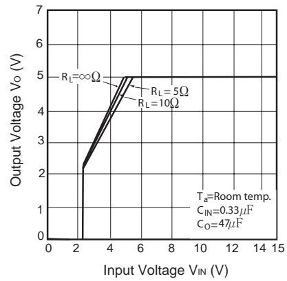
Fig.10 Output Voltage vs. Input Voltage (PQ050RDA1SZH)
