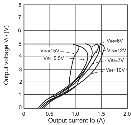
Fig.5 Overcurrent Protection Characteristics (PQ050RDA1SZH)
