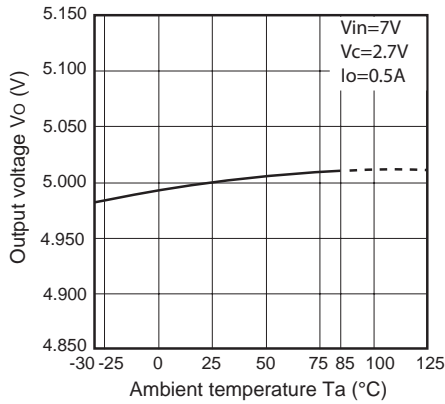
Fig.21 Output Voltage vs. Ambient Temperature (PQ050RDA1SZH)
