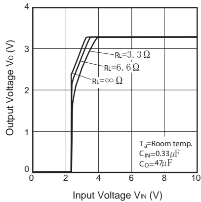
Fig.9 Output Voltage vs. Input Voltage (PQ033RDA1SZH)
