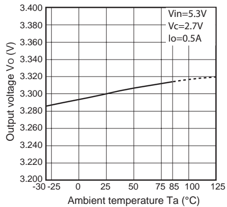
Fig.20 Output Voltage vs. Ambient Temperature (PQ033RDA1SZH)
