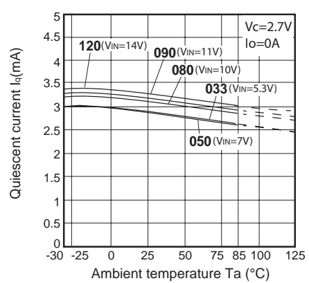
Fig.26 Quiescent Current vs. Ambient Temperature (PQxxxRDA1SZH)
