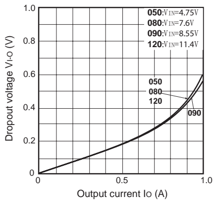
Fig.19 Dropout Voltage vs. Output Current (PQxxxRDA1SZH)
