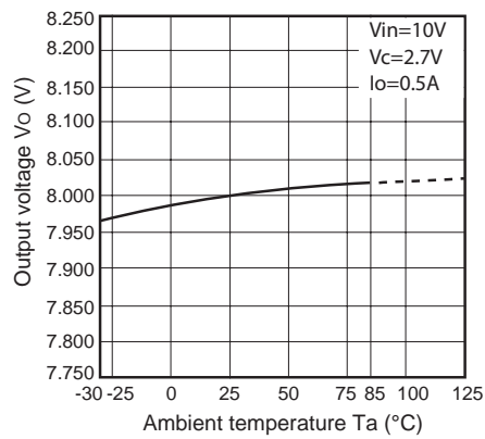
Fig.22 Output Voltage vs. Ambient Temperature (PQ080RDA1SZH)
