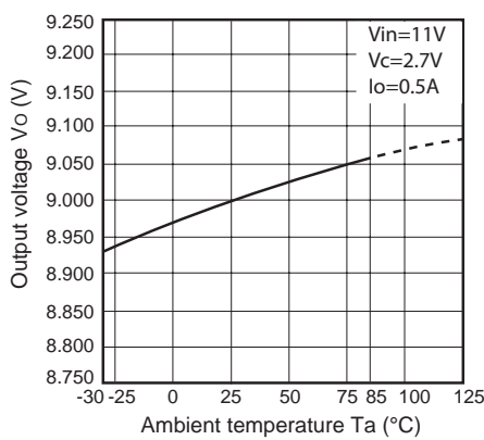
Fig.23 Output Voltage vs. Ambient Temperature (PQ090RDA1SZH)
