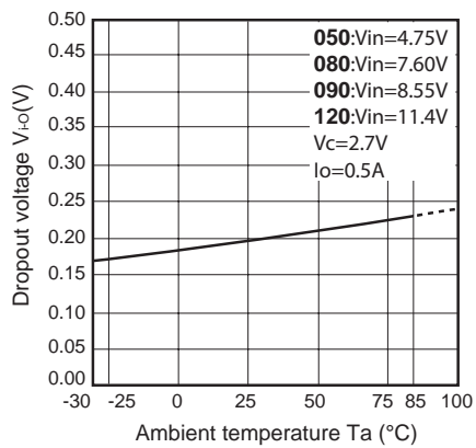
Fig.25 Dropout Voltage vs. Ambient Temperature (PQxxxRDA1SZH)
