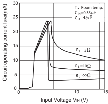
Fig.15 Circuit Operating Current vs. Input Voltage (PQ050RDA1SZH)
