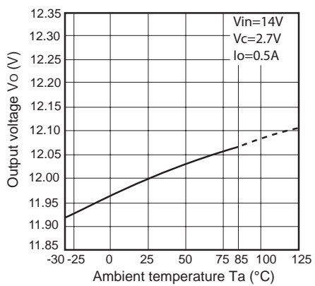
Fig.24 Output Voltage vs. Ambient Temperature (PQ120RDA1SZH)
