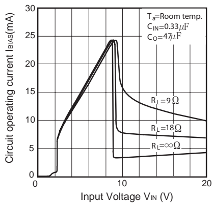
Fig.17 Circuit Operating Current vs. Input Voltage (PQ090RDA1SZH)
