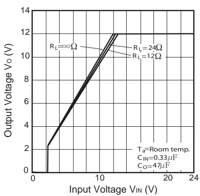
Fig.13 Output Voltage vs. Input Voltage (PQ120RDA1SZH)
