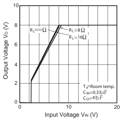
Fig.11 Output Voltage vs. Input Voltage (PQ080RDA1SZH)
