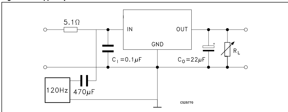
Figure 5. Ripple rejection
