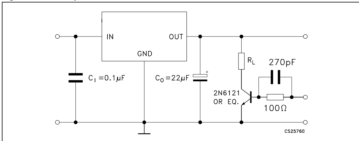
Figure 4. Load rejection
