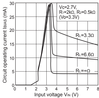
Fig.17 Circuit Operating Current vs. Input Voltage (PQ20WZ11J00H)
