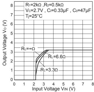
Fig.9 Output Voltage vs. Input Voltage (PQ20WZ11J00H)
