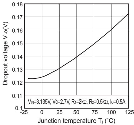
Fig.11 Dropout Voltage vs. Junction Temperature (PQ20WZ11J00H)
