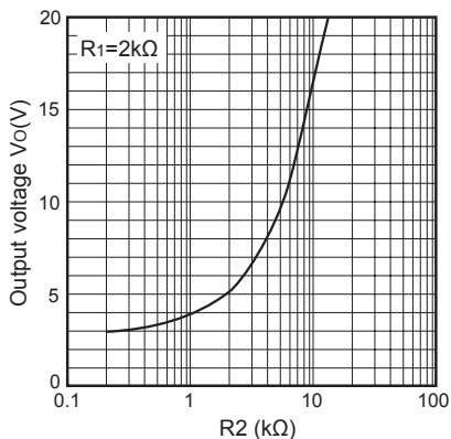
Fig.6 Output Voltage Adjustment Characteristics
