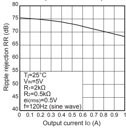
Fig.15 Ripple Rejection vs. Output Current (PQ20WZ11J00H)
