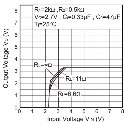
Fig.8 Output Voltage vs. Input Voltage (PQ20WZ51J00H)
