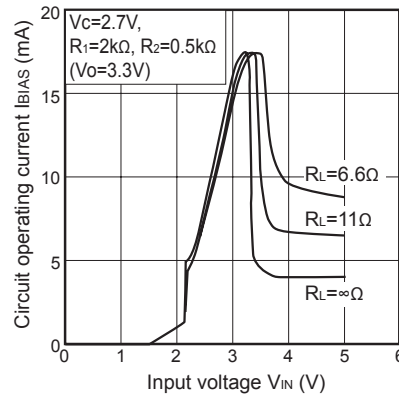
Fig.16 Circuit Operating Current vs. Input Voltage (PQ20WZ51J00H)
