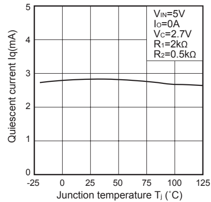
Fig.12 Quiescent Current vs. Junction Temperature
