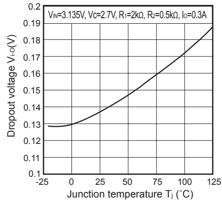
Fig.10 Dropout Voltage vs. Junction Temperature (PQ20WZ51J00H)
