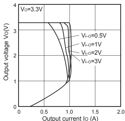
Fig.4 Overcurrent Protection Characteristics (Typical Value)(PQ20WZ51J00H)
