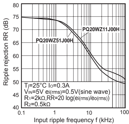
Fig.13 Ripple Rejection vs. Input Ripple Frequency
