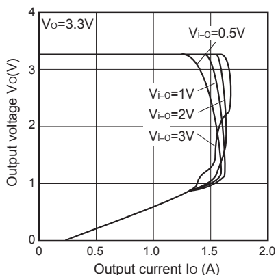
Fig.5 Overcurrent Protection Characteristics (Typical Value)(PQ20WZ11J00H)
