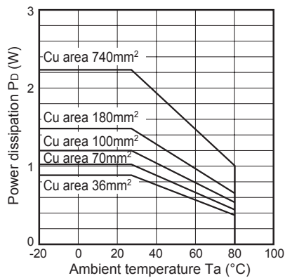
Fig.18 Power Dissipation vs. Ambient Temperature
