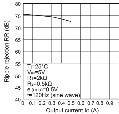
Fig.14 Ripple Rejection vs. Output Current (PQ20WZ51J00H)
