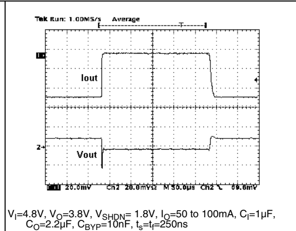
Figure 30. Load transient
