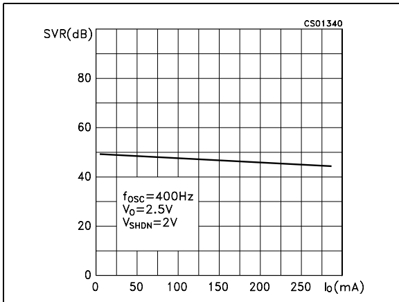
Figure 13. Supply voltage rejection vs. output current
