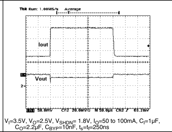
Figure 30. Load transient
