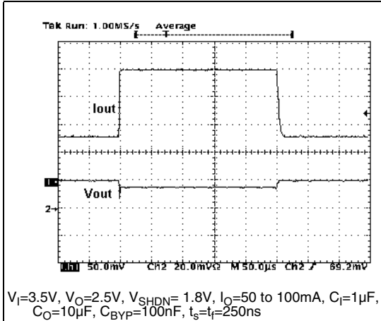
Figure 29. Load transient
