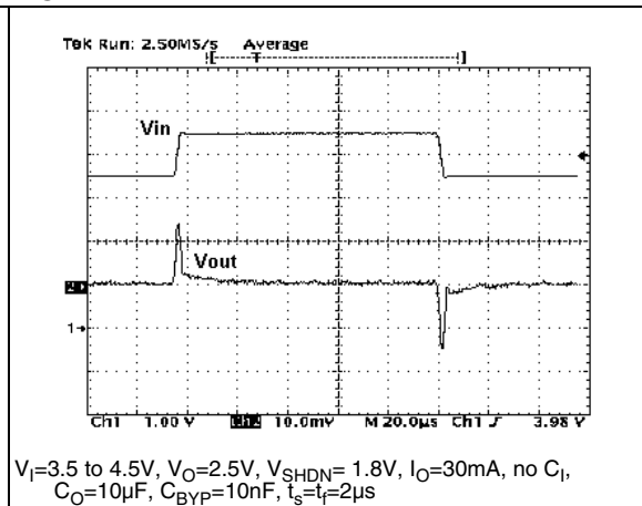
Figure 26. Line transient
