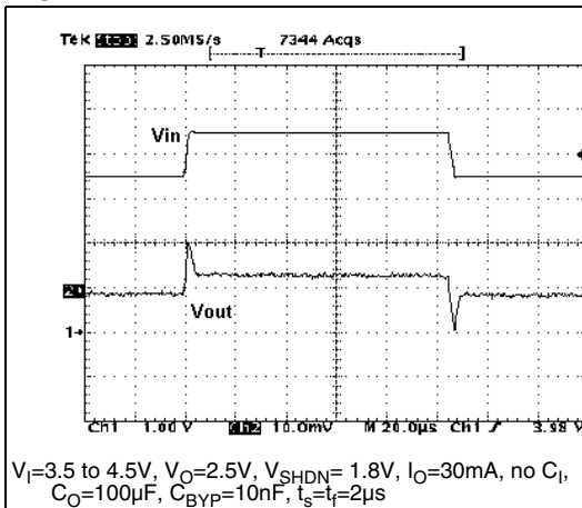
Figure 25. Line transient
