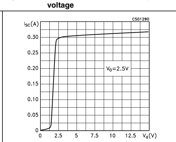
Figure 8. Short circuit current vs. dropout voltage
