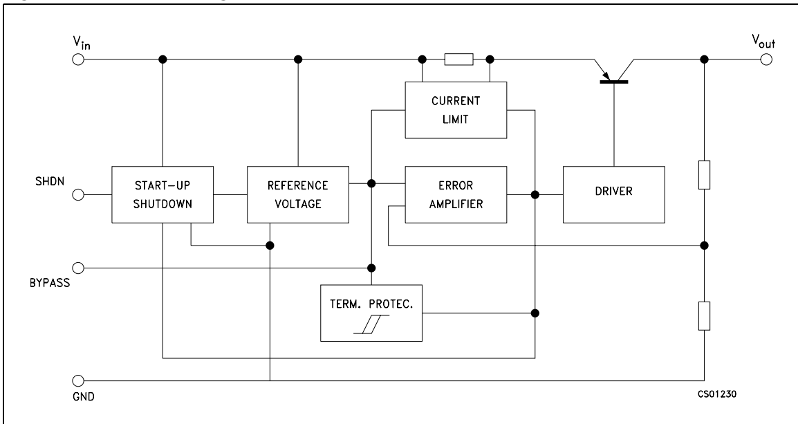
Figure 1. Schematic diagram
