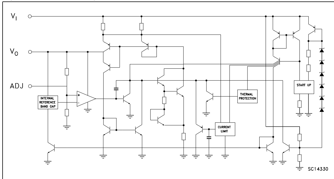
Figure 1. Schematic diagram
