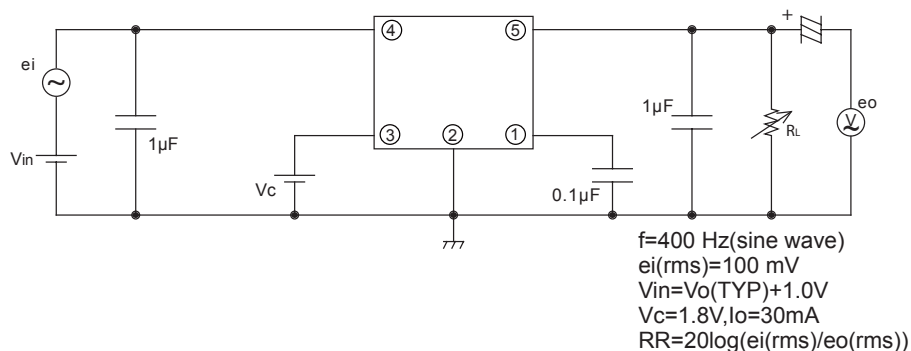
Fig.2 Test Circuit for Ripple Rejection
