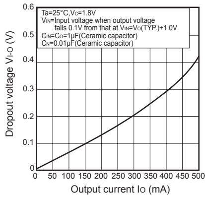
Fig.10 Dropout Voltage vs. Output Current (Typical Value)
