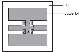
Mounting PCB
