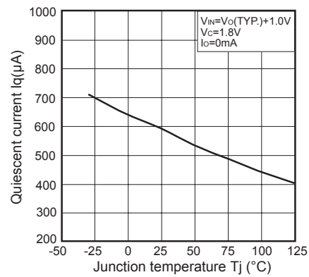
Fig.7 Quiescent Current vs. Junction Temperature (Typical Value)
