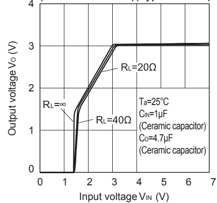
Fig.6 Output Voltage vs. Input Voltage (PQ1X301M2ZPH)(Typical Value)
