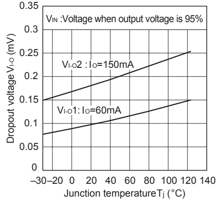
Fig.8 Dropout Voltage vs. Junction Temperature (PQ1X301M2ZPH)(Typical Value)
