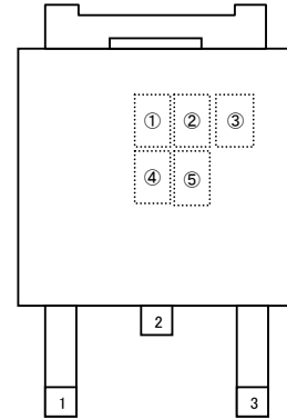
TO-252
