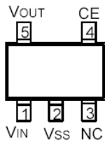
SOT-25 (TOP VIEW)
