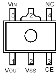
SOT-89-5 (TOP VIEW)
