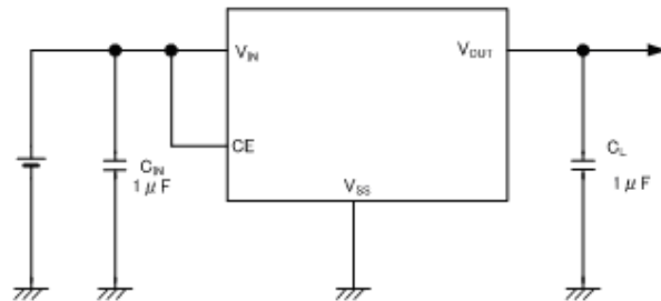
XC6701B Series With CE function
