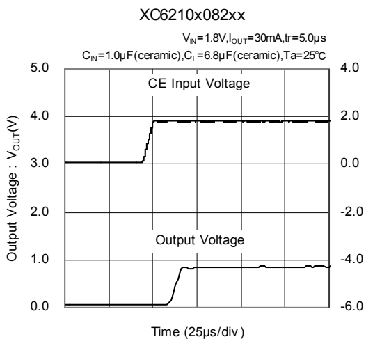
(11) Input Transient Response 2
