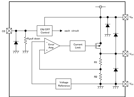
XC6210A Series
