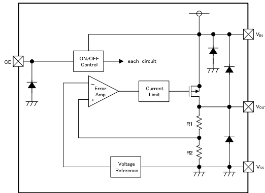
XC6210B/D Series
