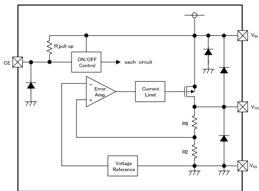
XC6210C Series
