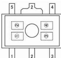
SOT-89-5 (TOP VIEW)
