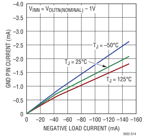
Negative Side GND Pin Current vs I LOAD
