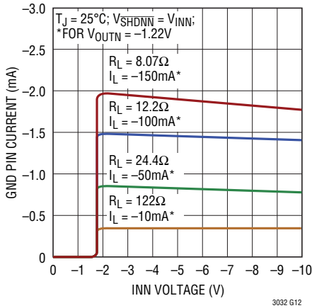
LT3032 Negative Side GND Pin Current
