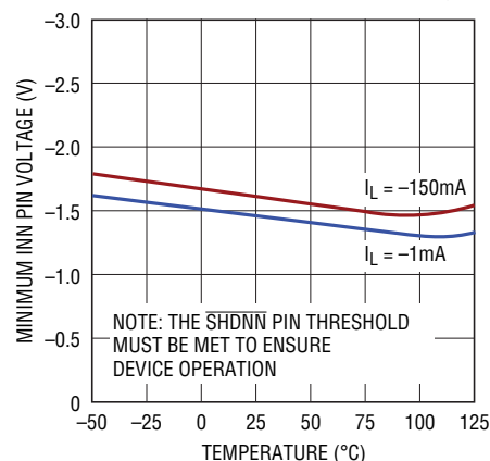
LT3032 Minimum INN Pin Voltage
