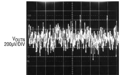
OUTN, 10Hz to 100kHz Output Noise, C_{BYPN} = 0
