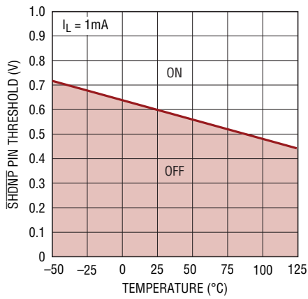
SHDNP Pin Threshold
