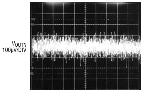
OUTN, 10Hz to 100kHz Output Noise, C_{BYPN} = 0.01\mu F
