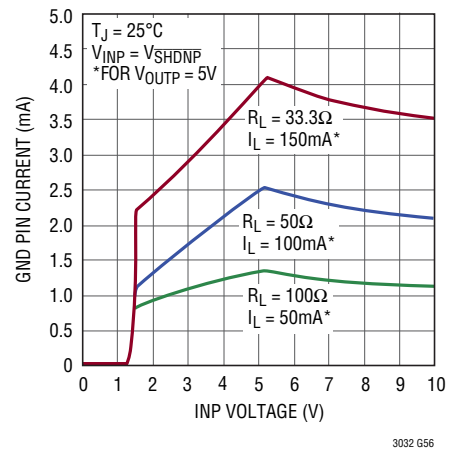
LT3032 Positive Side GND Pin Current
