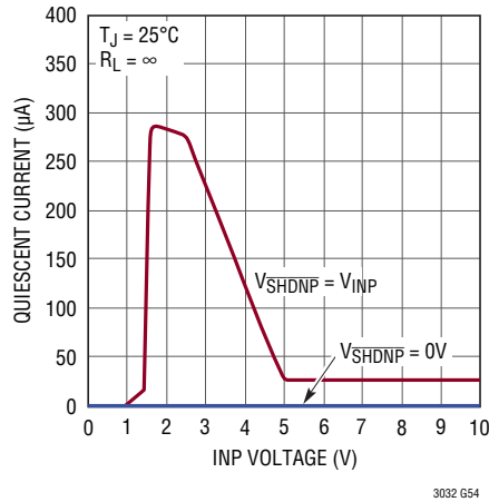
LT3032-5 INP Quiescent Current
