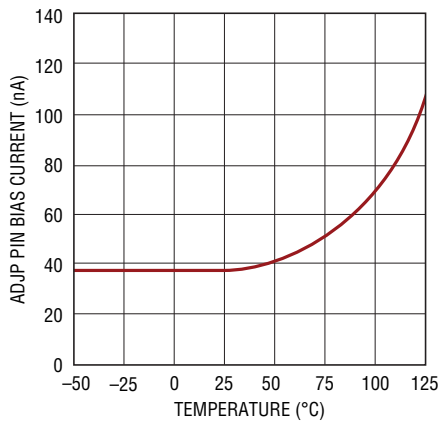
ADJP Pin Bias Current
