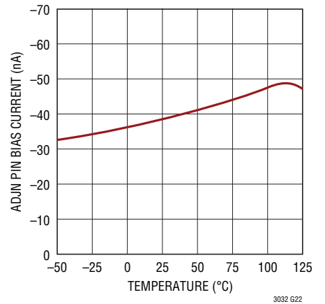
ADJN Pin Bias Current
