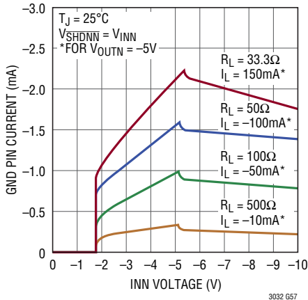
LT3032-5 Negative Side GND Pin Current
