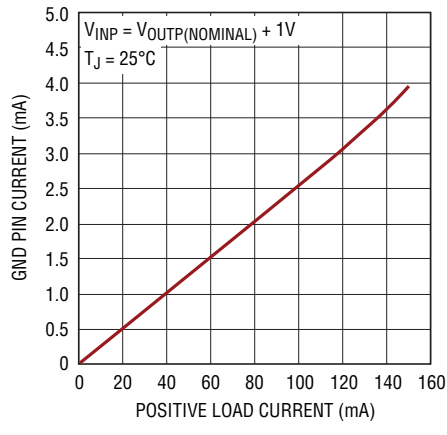
Positive Side GND Pin Current vs I LOAD
