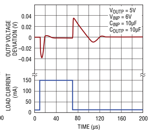
OUTP Transient Response C_{BYPP} = 0.01\mu F
