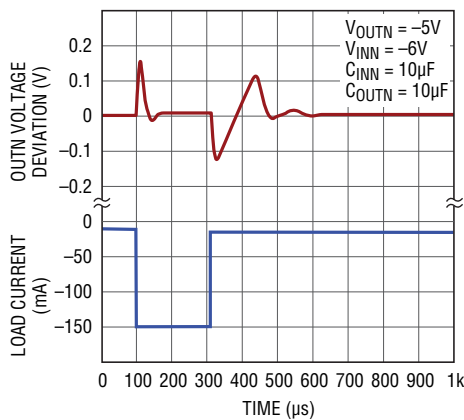
OUTN Transient Response C_{BYPN} = 0
