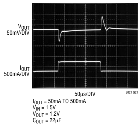
Transient Response
