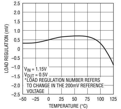
Load Regulation \Delta I_L = 1mA to 500mA
