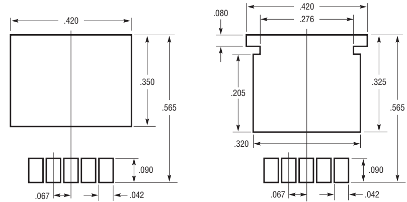
RECOMMENDED SOLDER PAD LAYOUT NOTE: 1. DIMENSIONS IN INCH/(MILLIMETER) 2. DRAWING NOT TO SCALE
