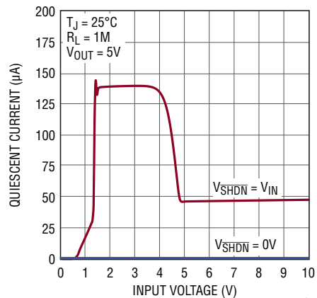
LT3060-5 Quiescent Current
