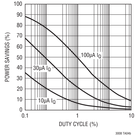
Average Power Savings for Low Duty Cycle Applications 0mA to 10mA Pulsed Load, I_N = 12V
