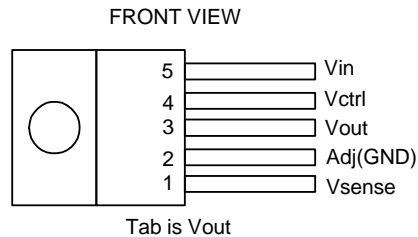
TO220-5L
