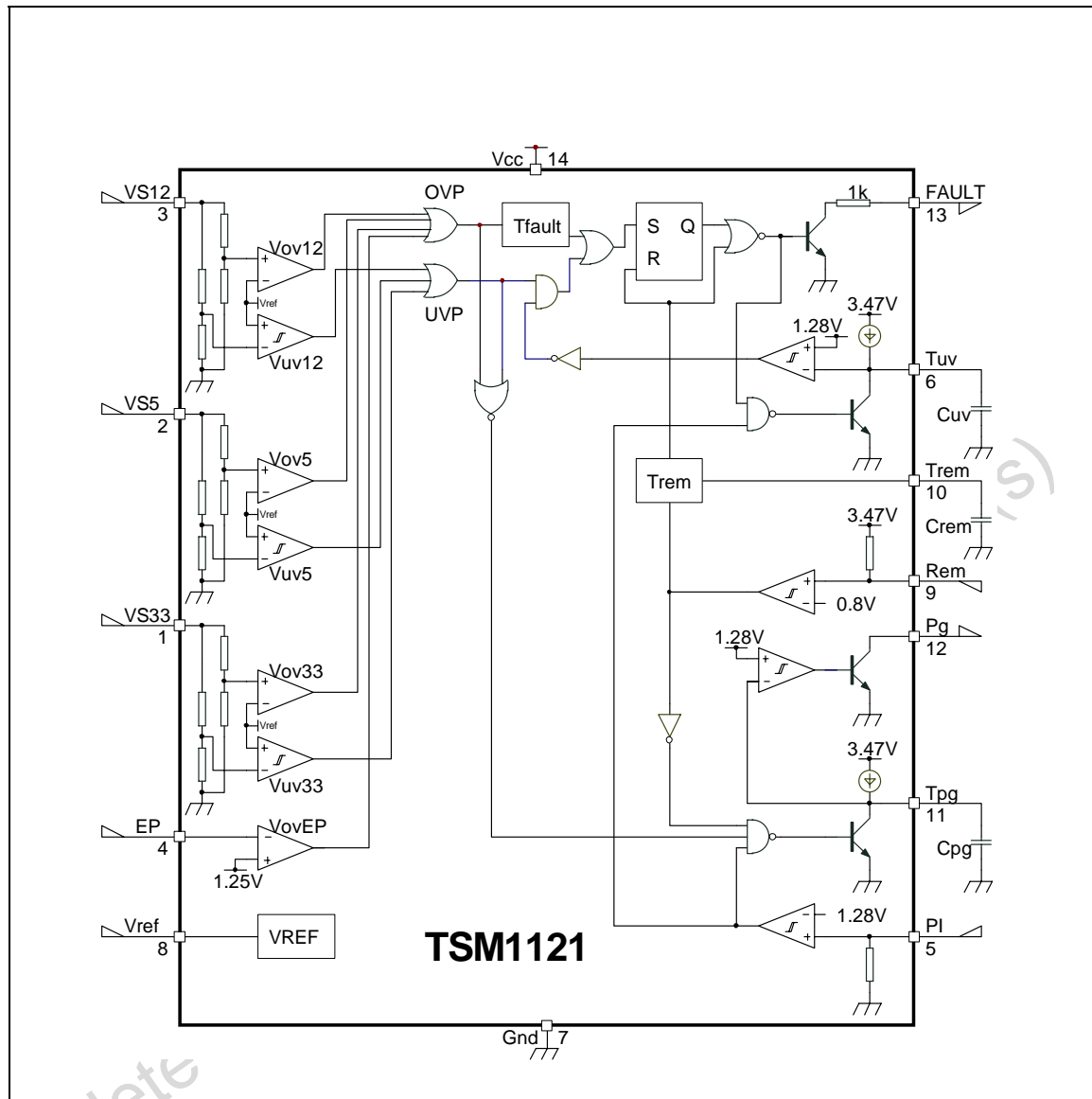
Fig. 3: Detailed Internal Schematic
