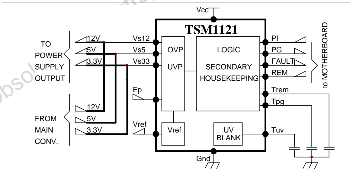
Fig. 2: Internal Schematic
