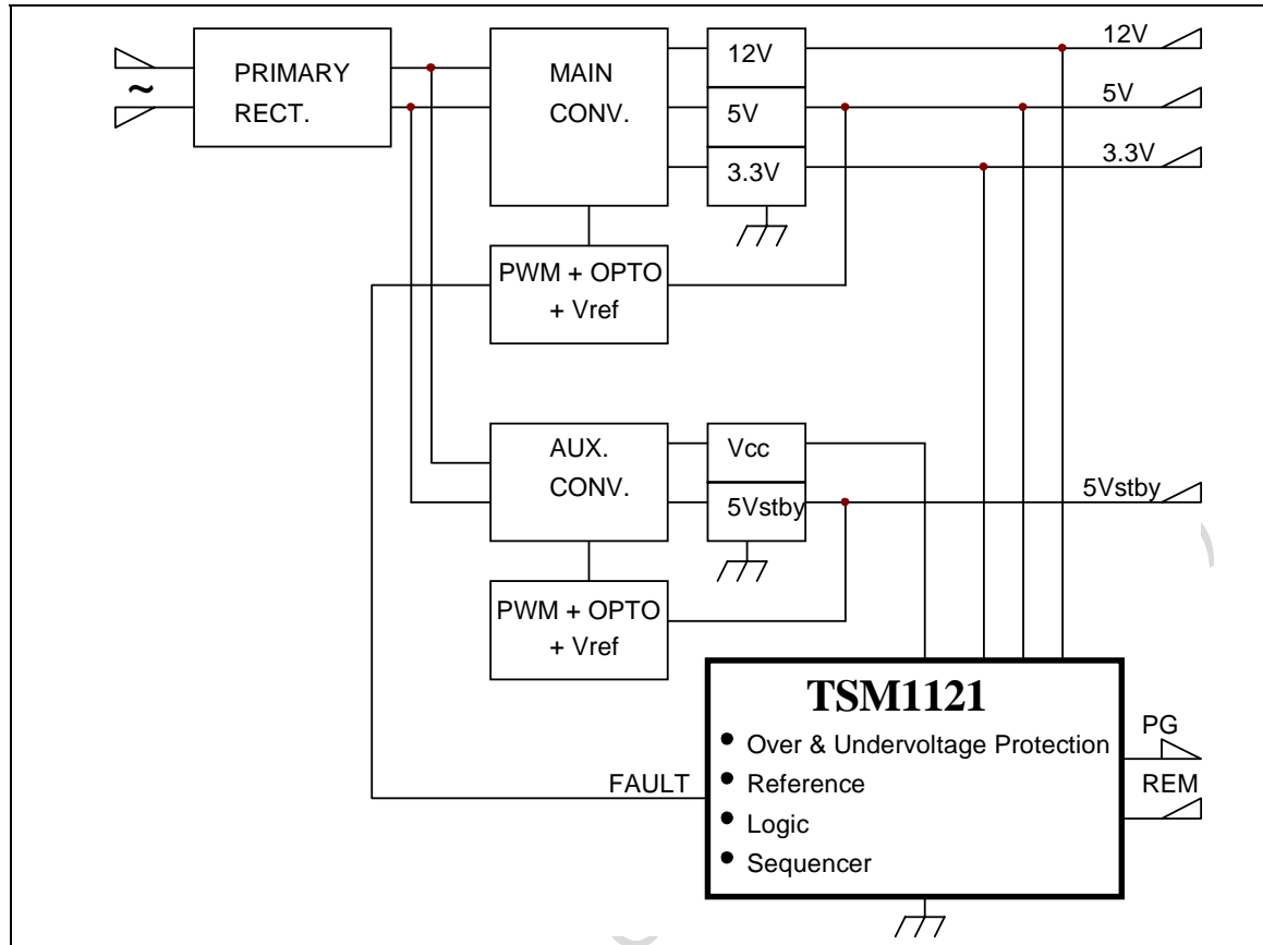
Fig. 2: Internal Schematic
