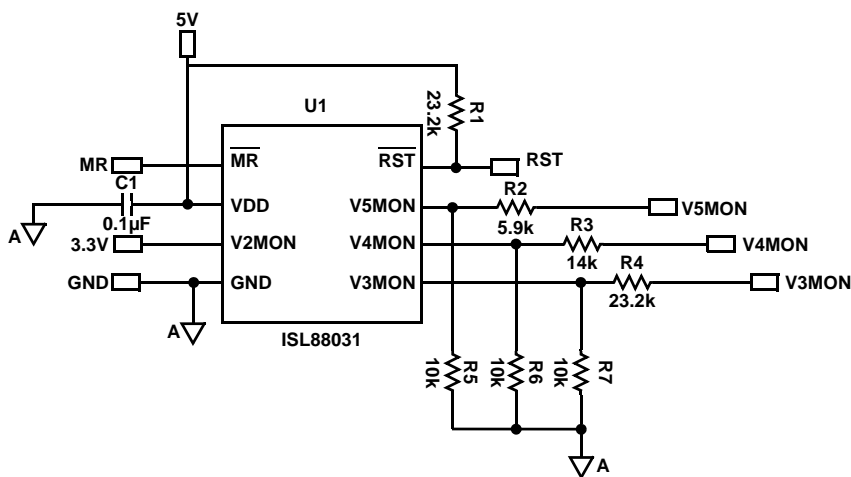
FIGURE 4. ISL88031EVAL1 SCHEMATIC AND PHOTOGRAPH
