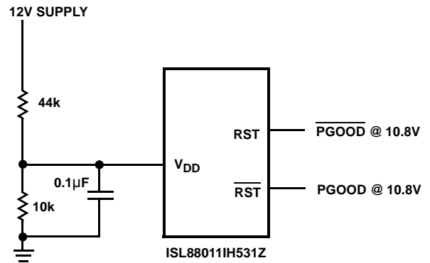
FIGURE 13. 12V SUPPLY PGOOD or \overline{PGOOD}
