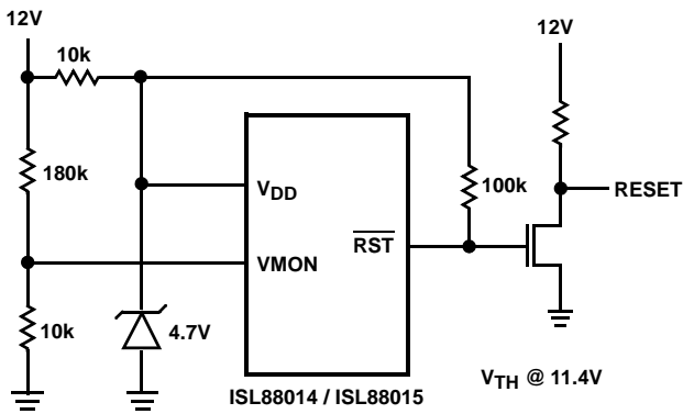
FIGURE 12. HIGH ACCURACY 12V SUPPLY MONITOR
