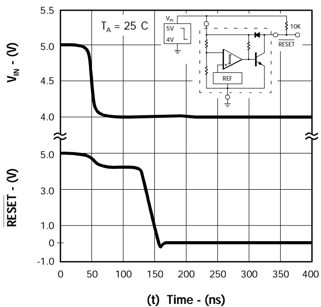
FIGURE 13. — PROPAGATION DELAY — HIGH to LOW
