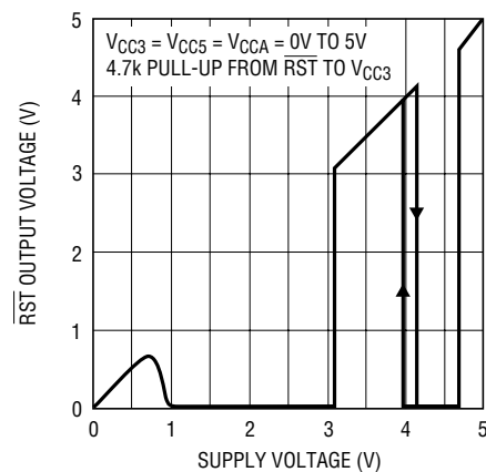
Figure 2. \overline{\text{RST}} Voltage vs Supply Voltage
